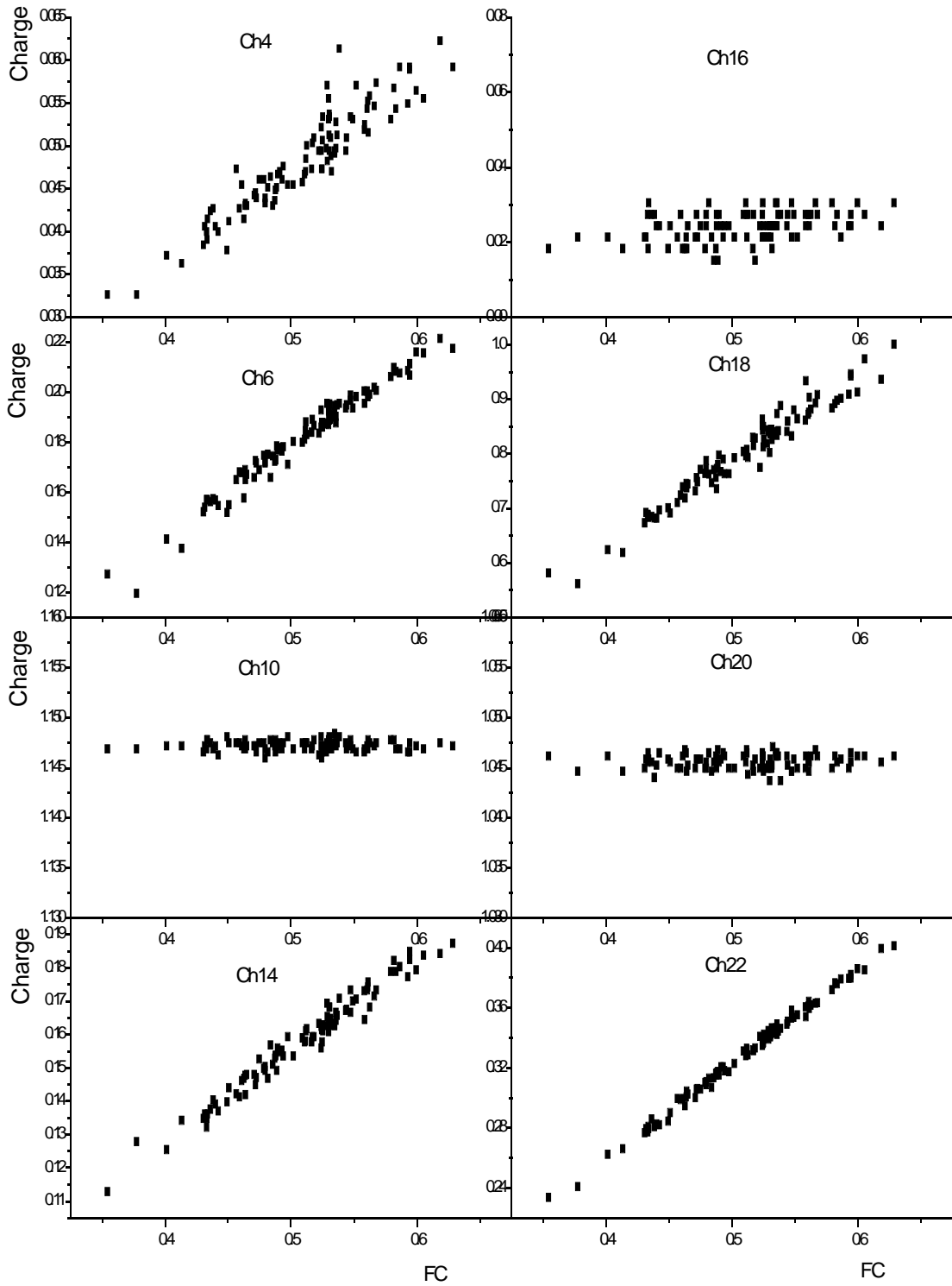
Channel Charge Vs. FCfor 206
