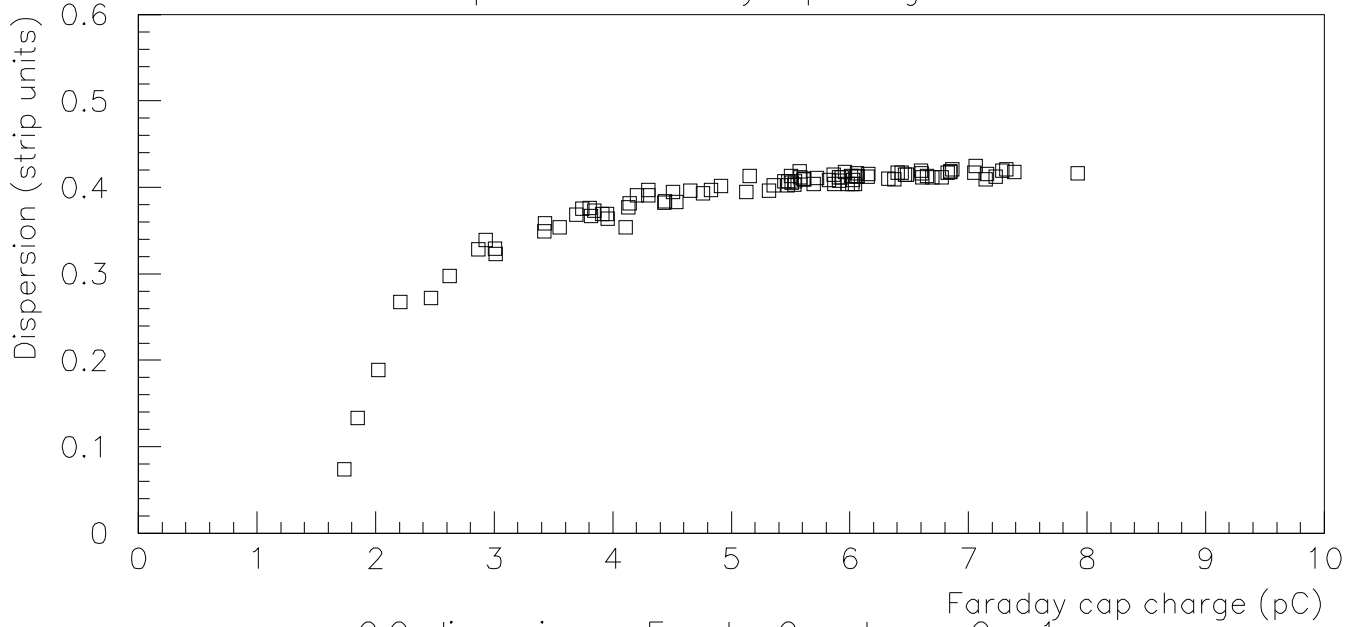
C.G. dispersion vs. Faraday Cap charge. Gap 1cm
