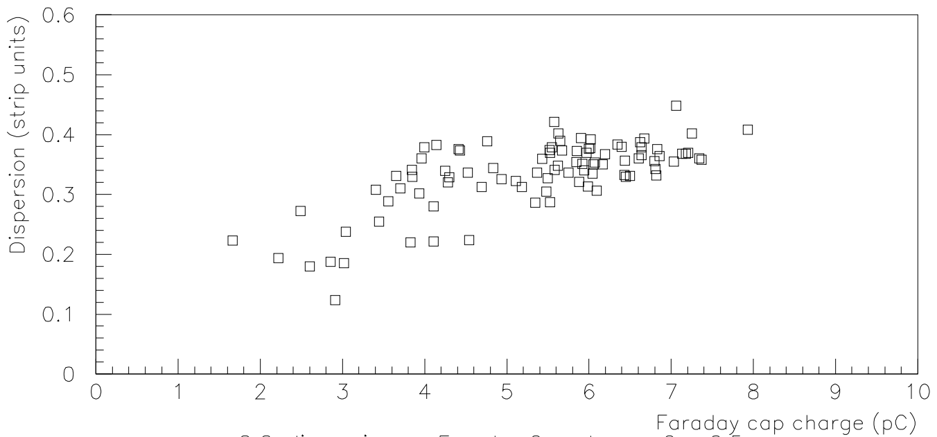
C.G. dispersion vs. Faraday Cap charge. Gap 0.5cm
